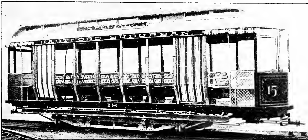
Fig. 5649. OPEN ELECTRIC-MOTOR CAR, WITH INCLOSED ENDS AND STEAM CAR ROOF. Length over all, 30 ft. No. 6E Peckham Trucks. JACKSON & SHARP COMPANY, WILMINGTON, DELAWARE.
